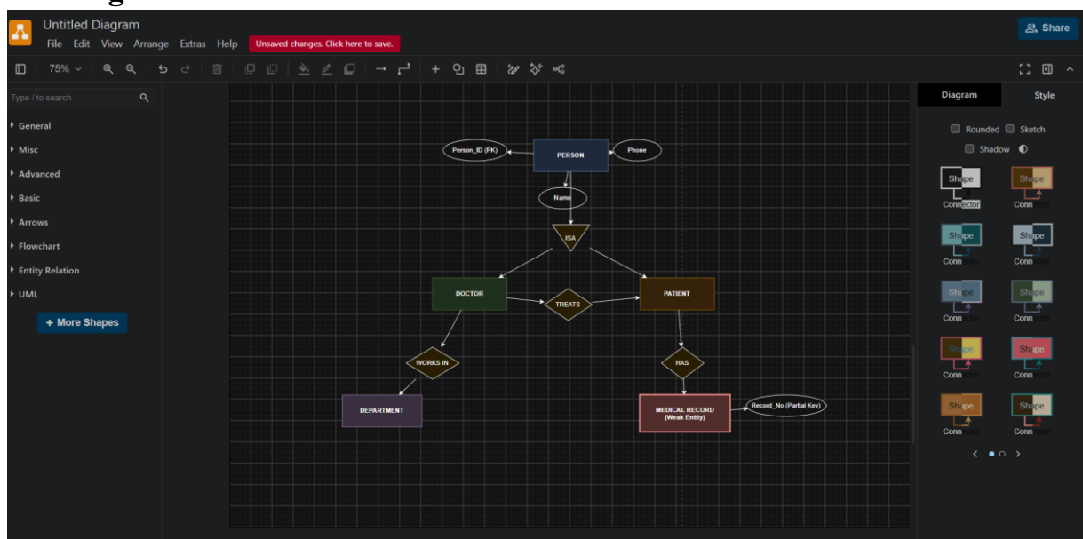
Fig.5: Hospital Data Explanation of the EER Diagram
